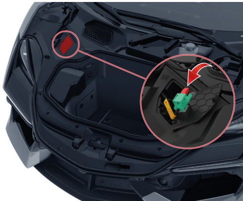
Disconnect high voltage device in the frunk of Revuelto and Temerario
