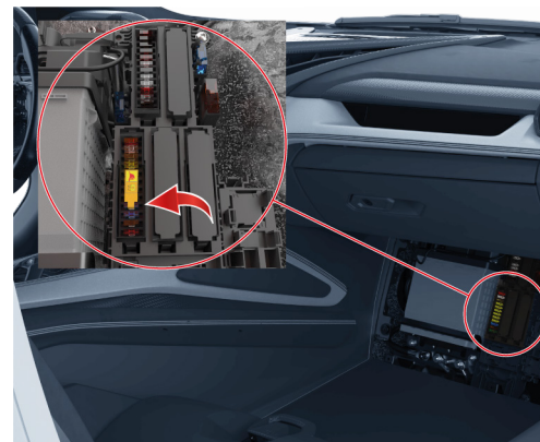
Disconnect high-voltage device (fuse) of Revuelto and Temerario located in the fuse panel in the passenger compartment
